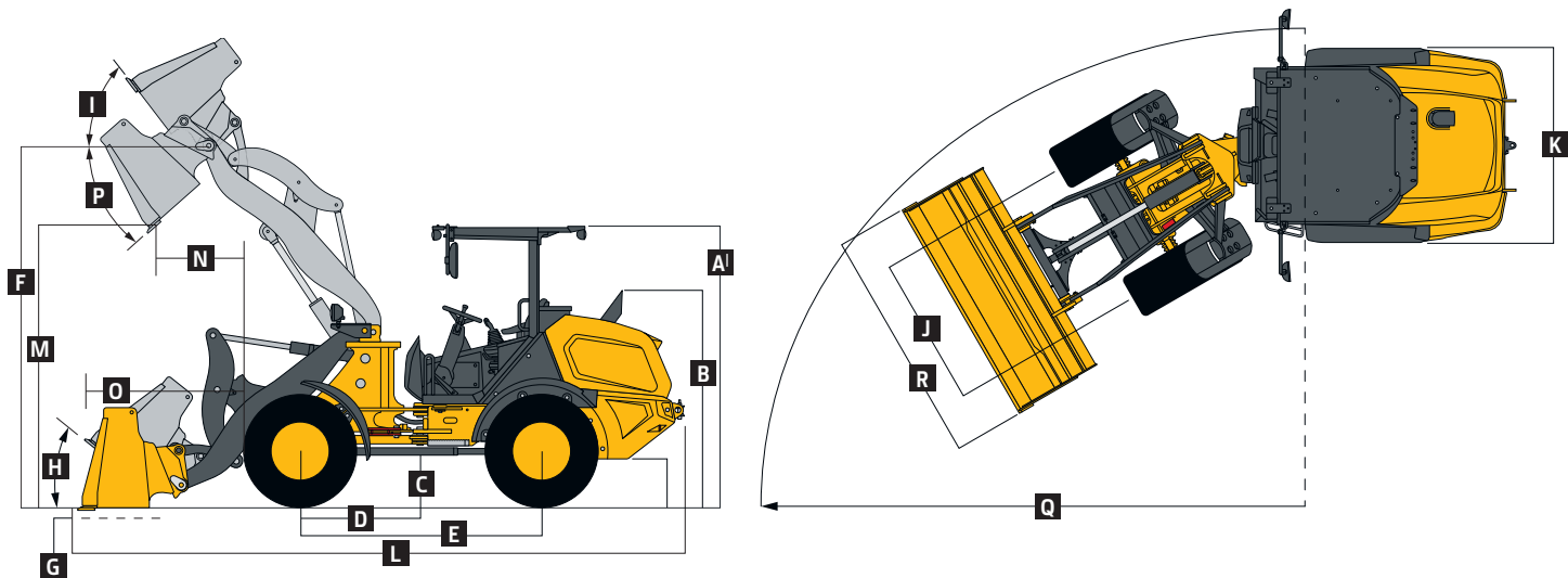
204 G-TIER LOADER WITH CANOPY, QUIK-TATCH COUPLER OR HOOK/EURO QUICK-COUPLER, AND BUCKET
