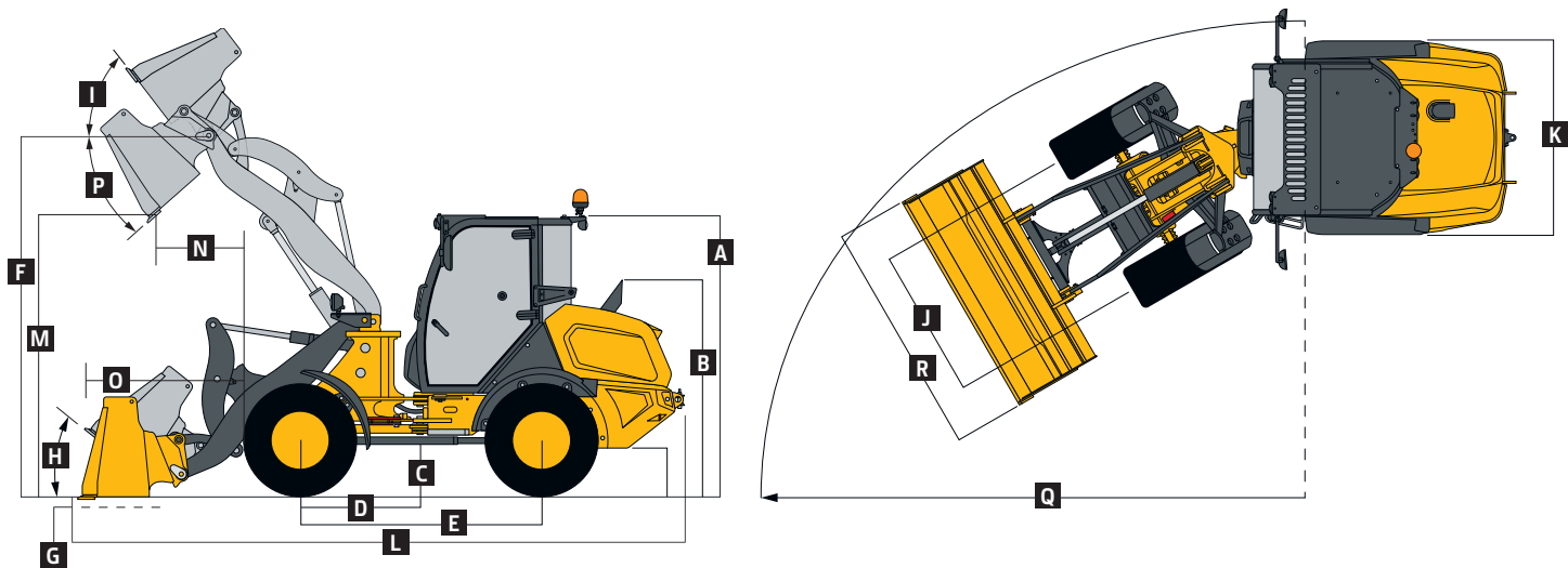
204 G-TIER LOADER WITH CAB, QUIK-TATCH COUPLER OR HOOK/EURO QUICK-COUPLER, AND BUCKET
