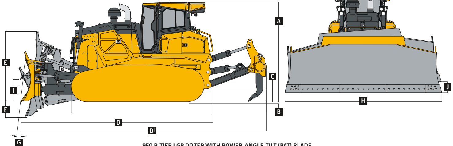
950 P-TIER LGP DOZER WITH POWER-ANGLE-TILT (PAT) BLADE
